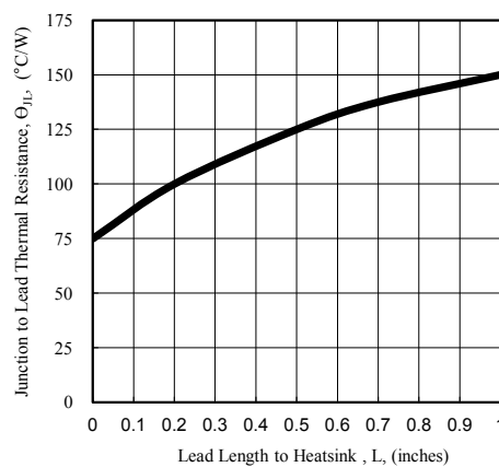
Fig. 3 - Typical Thermal Resistance v.s. Lead Length
