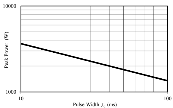
Fig. 4 - Peak Pulse Power Rating Curve
