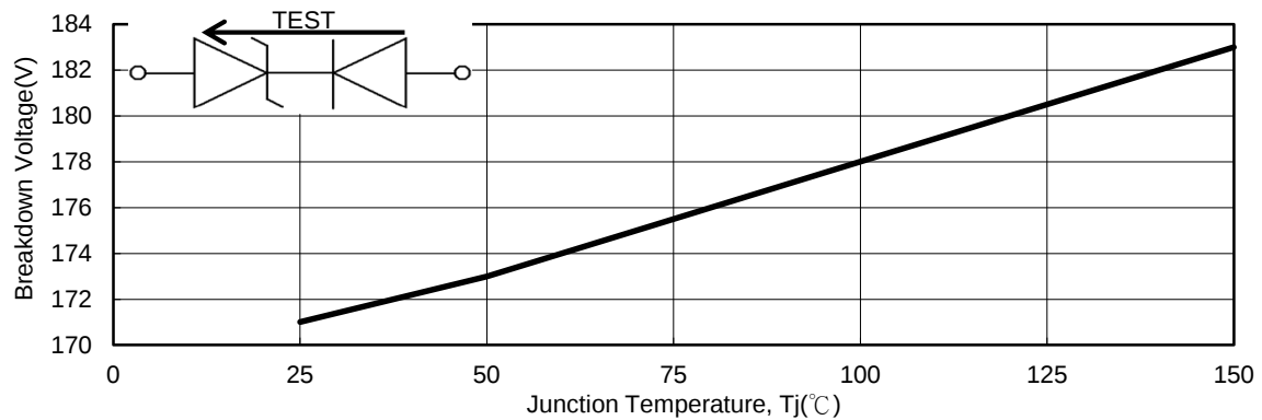
Fig.2 - Breakdown Voltage
