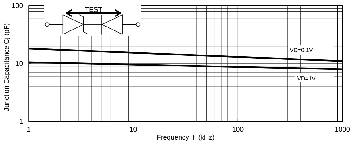
Fig.1 - Junction Capacitance
