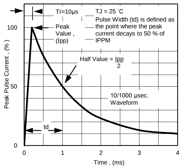
Fig.4 - Pulse Waveform
