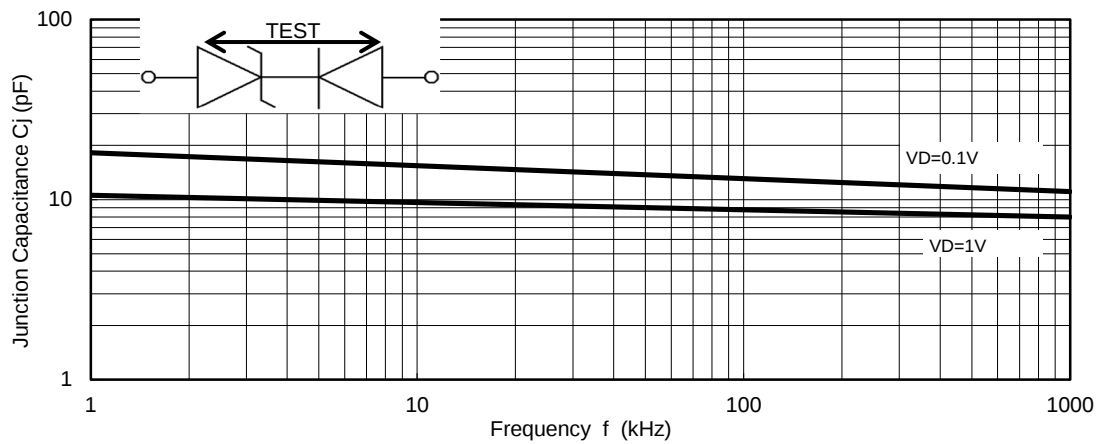
Fig.1 - Junction Capacitance
