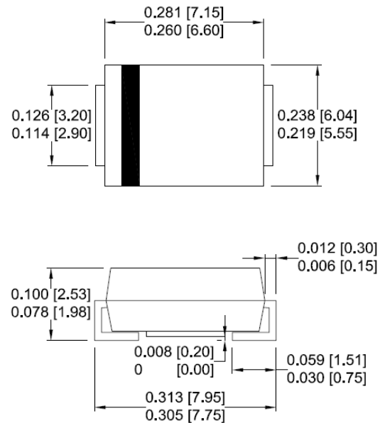
SMC/ DO-214AB
