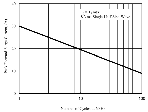
Fig. 2 - Maximum Non-Repetitive
